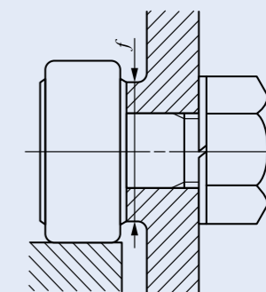
Fig.1 Seating surface
