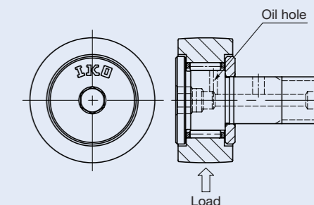
Fig.2 Oil hole position and loading direction
